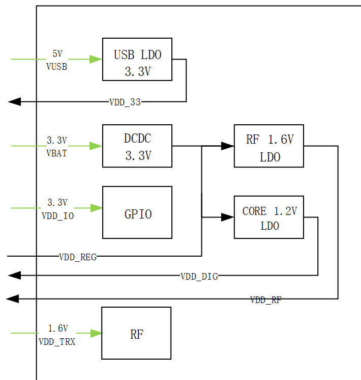
Figure 5 FS3101 Power DC
