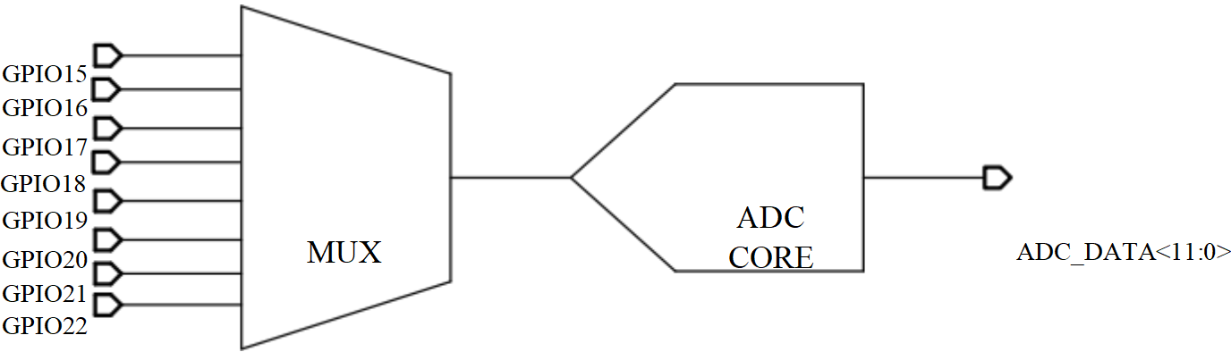
Figure 3 ADC signal path
