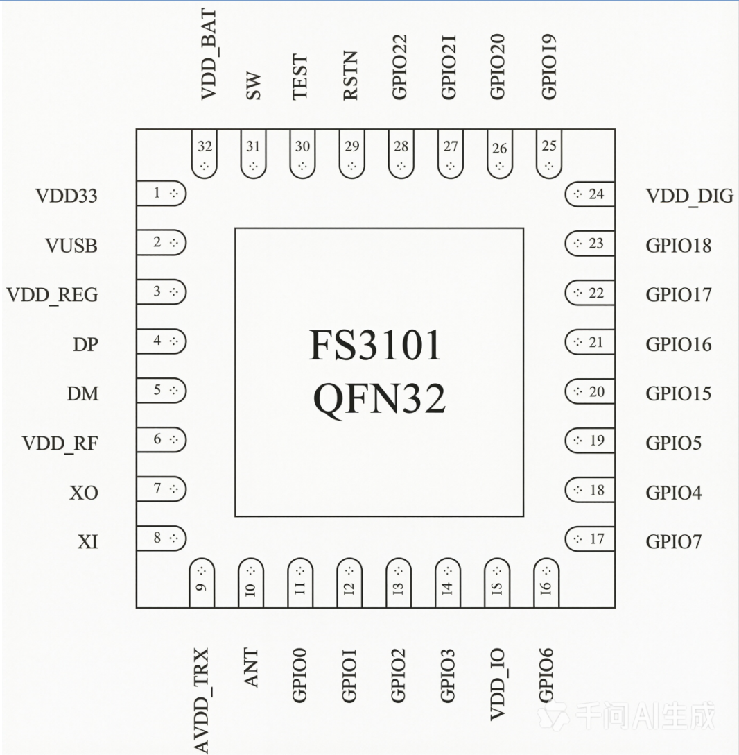
Figure 2: QFN32 Package PIN Diagram
