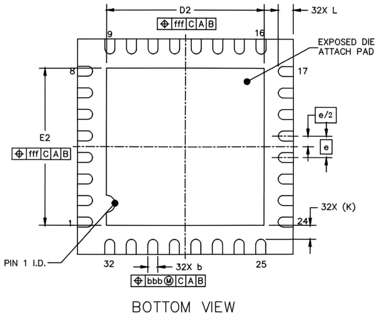
Figure 9 Package Dimension
