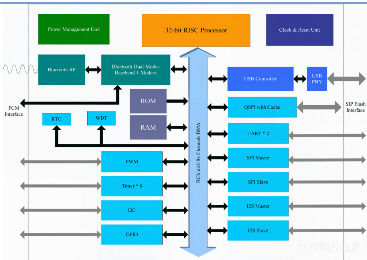
Figure 1: FS3101 Functional Block Diagram
