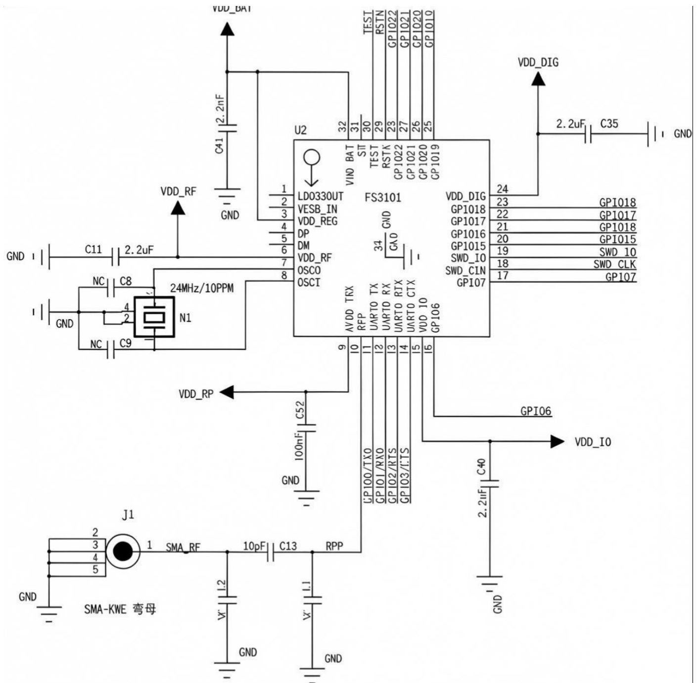
Figure 8 Reference circuit without DCDC
